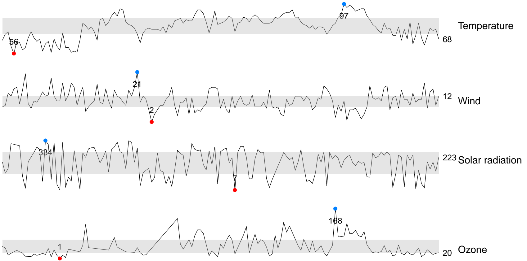
Daily changes of airquality and weather indices between May 1, 1973 and September 30, 1973
